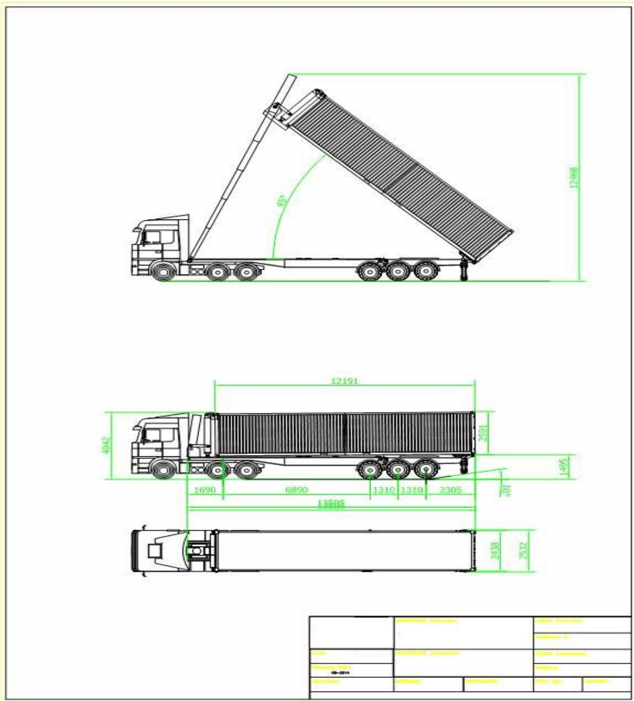
Pic. 7: 40' ISO Container Handling Unit ContiLift CHU-40 – Tilting/Dimensions
