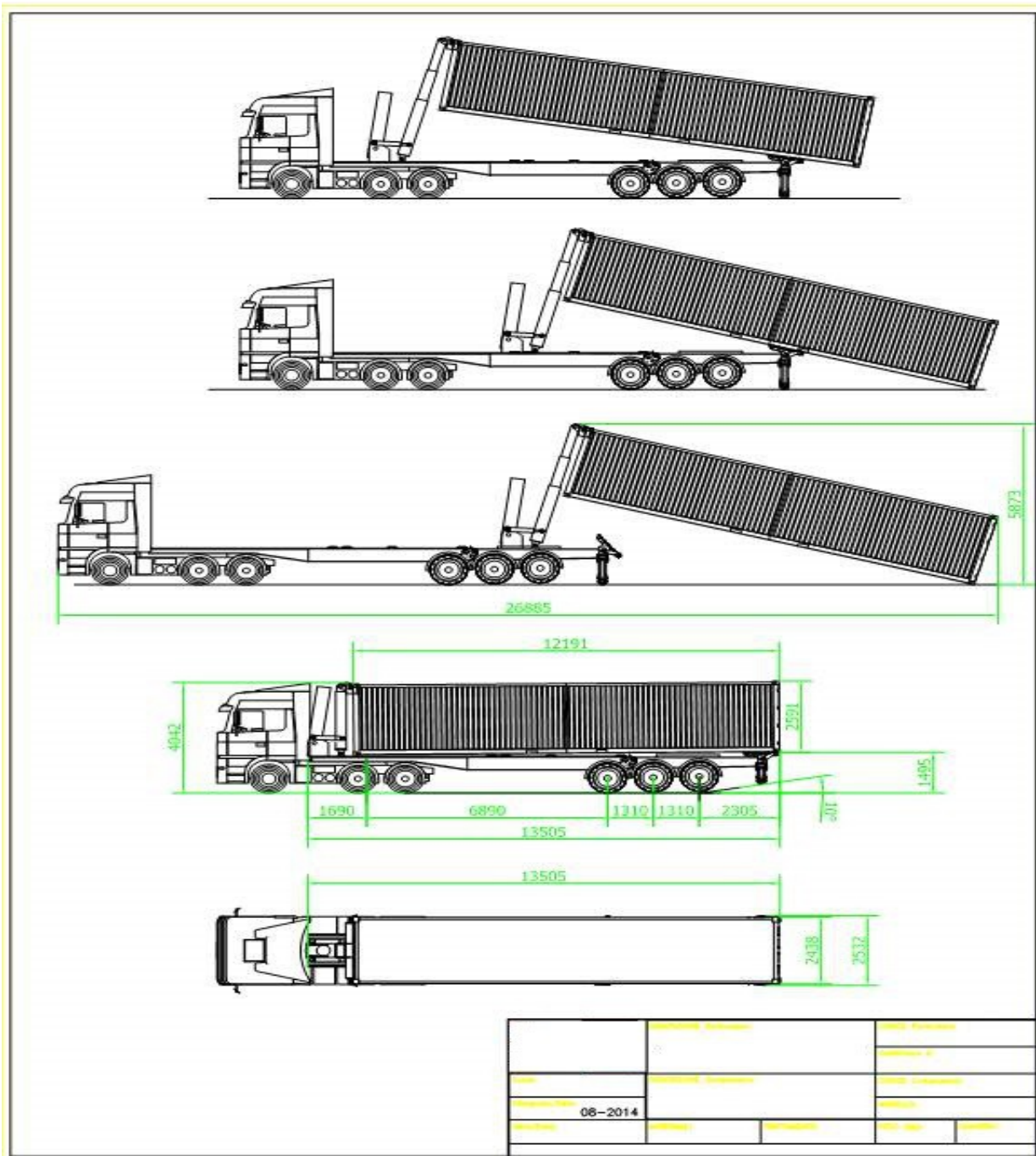
Pic. 6: 40' ISO Container Handling Unit ContiLift CHU-40 – Loading/Dimensions
