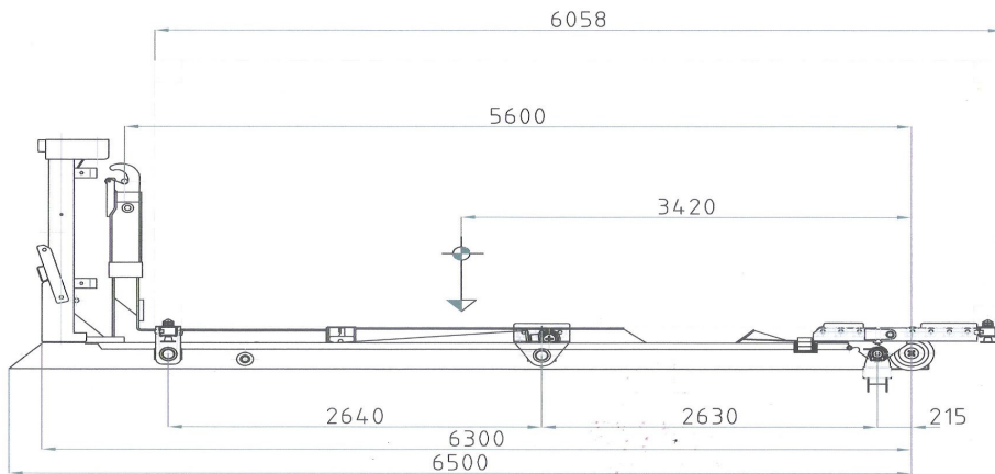
Pic. 6: ContiLift Hook Lift Module with 20' ISO Adapter ICAK-20-H/Technical Drawing
