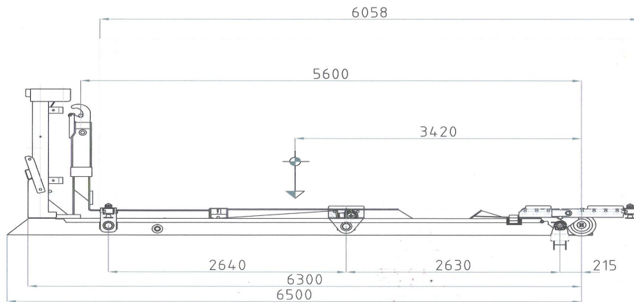
Pic. 6: EOS-ENVIRO Hook Lift Module with 20' ISO Adapter/Technical Drawing
